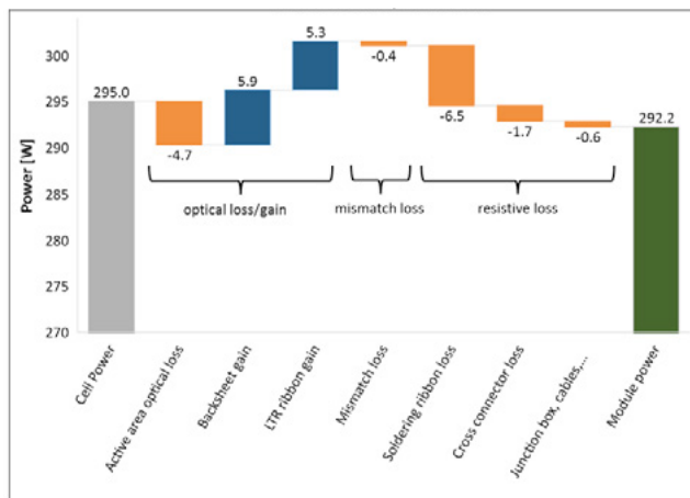
Cell-to-module (CTM) power loss analysis at SERIS
